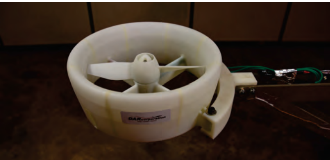
In-house 3D Printed Ducted Fan on Test Stand
