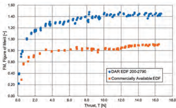
Thrust and Figure of Merit Comparison between In-house 3D Printed Ducted Fan (DAR EDF 200-2790) and Commercially Available Ducted Fan
